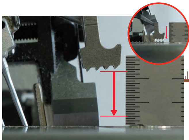
• Top feed vertical movement 9.5mm
